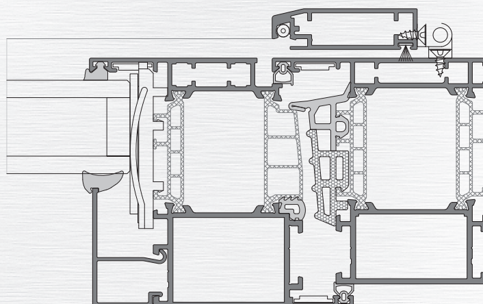
Horizontal cross-section - opening mosquito net
