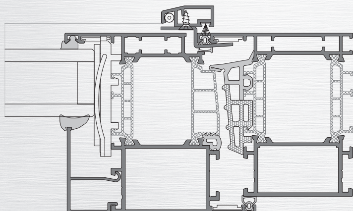
Horizontal cross-section - fixed mosquito net
